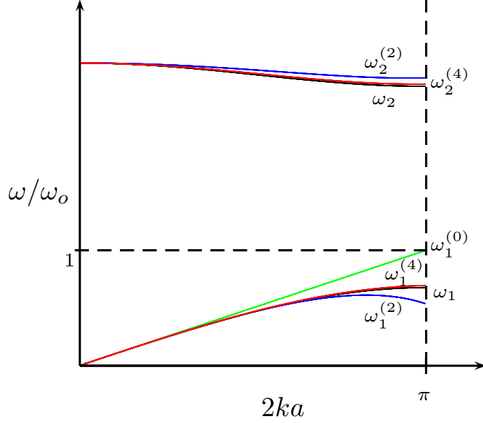
Figure 4: Exact dispersion curve (two branches (\omega_{1,2}) , in black) compared to its classical quasistatic approximation of order 0 (one branch (\omega_1^{(0)}) , in green), to its second-order approximation by the present theory (two branches (\omega_{1,2}^{(2)}) , in blue) and to its fourth-order approximation by the present theory (two branches (\omega_{1,2}^{(4)}) , in red).
