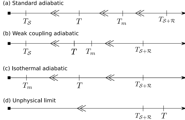
Figure 3: The different time-scale orderings of the adiabatic theorems. In the ordering (a) of the standard adiabatic theorem, the relevant evolution is that of the system \mathcal{S} with its associated time-scale T_{\mathcal{S}} . The ordering (c) is associated to the isothermal adiabatic theorem. The ordering for the weak coupling adiabatic theorem (b) is similar with the constraint T \sim \lambda^{-2} . In both cases the relevant time-scale is the thermalization time T_m . The ordering (d) corresponds to the unphysical limit where T is taken to infinity before the thermodynamic limit.
