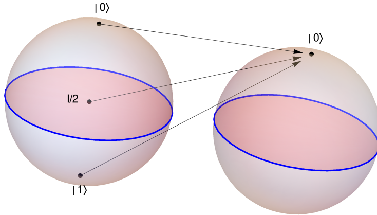
Figure 1: An erasure process maps the Bloch ball, the phase space of a qubit, into a single pure state, e.g., the point |0\rangle . A measurement of the qubit after erasure would not provide any information about the initial state. Since a general quantum operation transforms the Bloch ball into a (possibly degenerate) ellipsoid centered at the image of I/2 , a process is an erasure process if and only if it maps the completely mixed state I/2 into a pure state.
