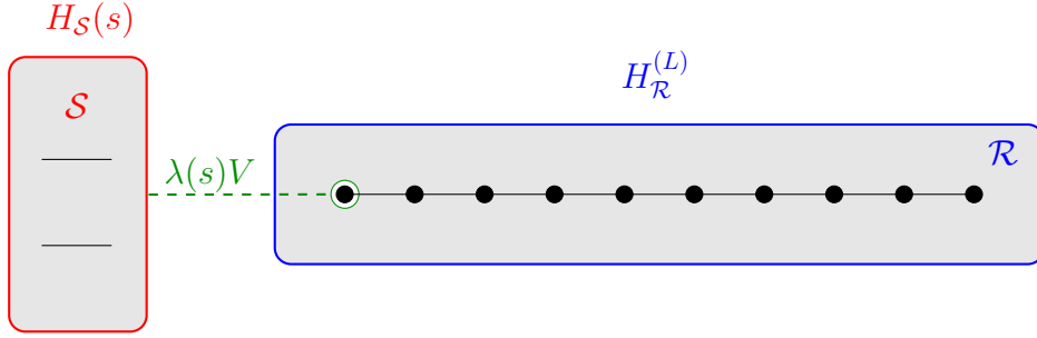
Figure 2: A 2-level quantum system \mathcal{S} interacts with a gas of fermions \mathcal{R} on a one dimensional lattice of size L . The epoch-dependent interaction \lambda(s)V couples \mathcal{S} to the fermions on the first site of this lattice.
