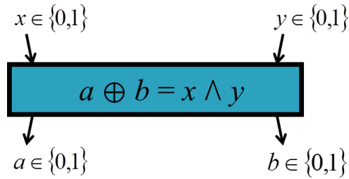
Figure 9. Boîte non-locale PR.
