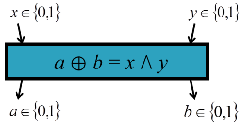
Figure 9. Boîte non-locale PR.
