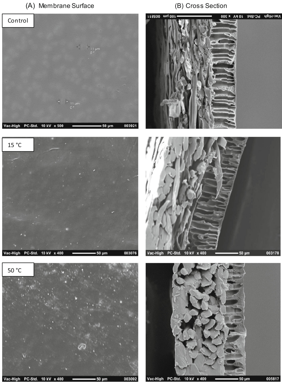
Fig. 7 The SEM images of membrane surface and cross section of new membrane (a), after skim milk ultrafiltration at 15 °C (b) and at 50 °C (c)
