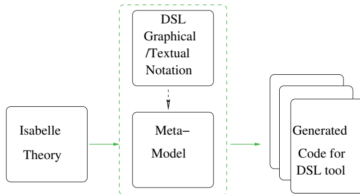
Fig. 5. Datatype To Ecore implementation architecture
