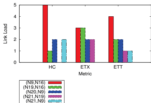
Fig. 5: Link Load.
