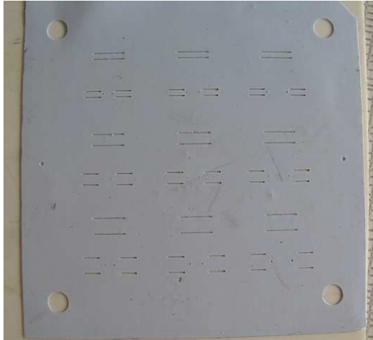
Figure 6: Prototype 1. The sixth layer after cutting the grooves with the micromachining laser. The tape size is 50.8 \times 50.8 \text{ mm}^2 . The four circular holes in the corners are for alignment on the stacking fixture, and the two smaller holes at half the substrate height are used for alignment during screen printing.
