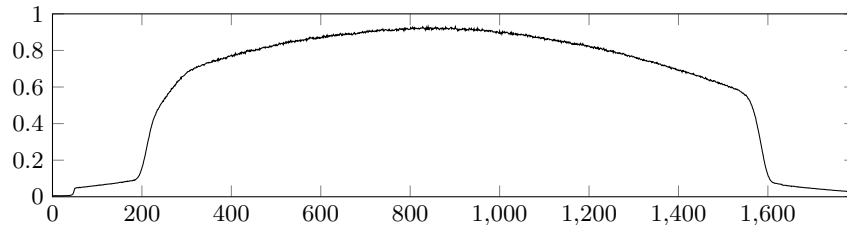
Fig. 4: Horizontal intensity profile of the fluence map for 120kV with a source cone angle of 50 deg.
