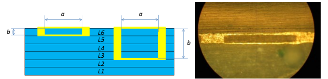
Fig. 3. Left: Layer stack for one and four-layered GLWG having an inner height of 75 and 300 \mu\text{m} respectively Right: Micrograph of cross-section of one of the one-layered G-band GLWGs. The inner dimension is found to be 610 \times 75 \mu\text{m} at the position of the cut. The gold filled grooves are 180 \mu\text{m} wide. Measurement tolerance is \pm 5 \mu\text{m} . LTCC is filling the portion below the GLWG in the micrograph.
