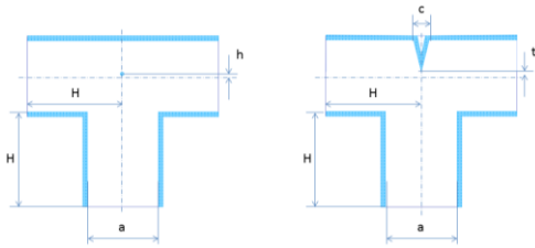
Fig. 8. U-band tee dimensions; a=2250\mu\text{m} , H=3000\mu\text{m} , h=75\mu\text{m} , t=135\mu\text{m} and c=500\mu\text{m} . The waveguides' inner height is 75\mu\text{m} . Left; the tee with the via, Right; tee with peaked groove.
