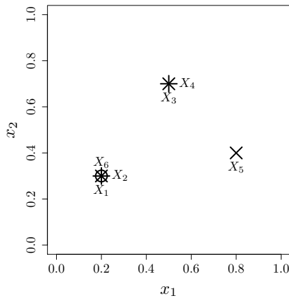
Figure 10: Kernel and DoE of the repeated points example
