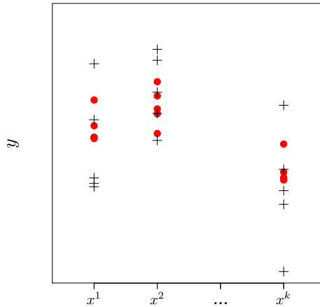
Figure 3: The response values \mathbf{y} and \mathbf{y}^+ are denoted by bullets and crosses, respectively. At each location, the mean of \mathbf{y} and \mathbf{y}^+ are identical, \bar{y}_i = \overline{y^+}_i , but the spread of observations in \mathbf{y}^+ is never less than that of \mathbf{y} at redundant points.
