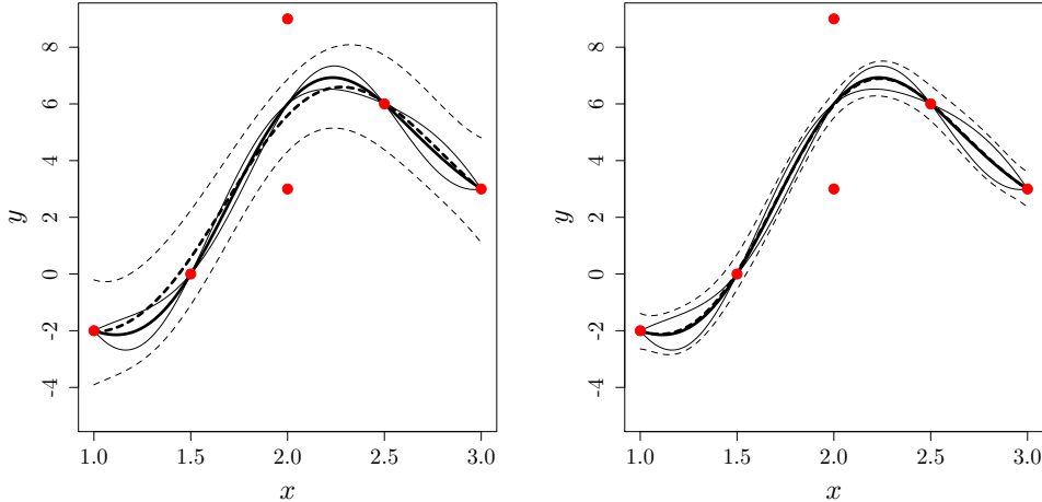
Figure 6: One dimensional kriging regularized by PI (solid lines) and nugget (dashed lines). The nugget amplitude is 1 on the left and 0.1 on the right. The cut-off eigenvalue for the pseudoinverse is \tau = 10^{-3} . m^{Nug}(x) is not interpolating which is best seen at the second point on the left. On the right, the PI and nugget models are closer to each other. Same \mathbf{X} and \mathbf{y} as Figure 4.
