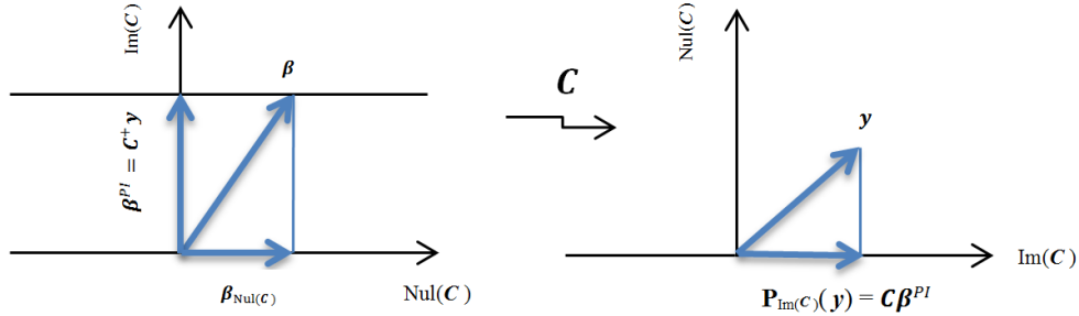
Figure 1: Geometrical interpretation of the Moore-Penrose pseudoinverse. In the leftmost picture, infinitely many vectors \beta are solutions to the system \mathbf{C}\beta = \mathbf{y} . But the minimum norm solution is \mathbf{C}^\dagger \mathbf{y} . The rightmost picture shows the orthogonal projection of \mathbf{y} onto the image space of \mathbf{C} , \mathbf{P}_{Im(\mathbf{C})}(\mathbf{y}) , which is equal to \mathbf{C}\mathbf{C}^\dagger \mathbf{y} (Property 1).
