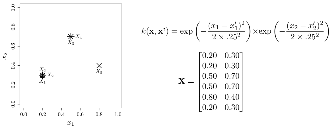
Figure 9: Kernel and DoE of the repeated points example
