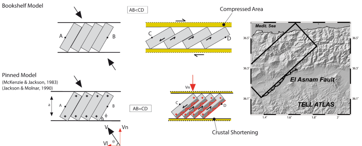
Figure 4. Upper panels: Kinematic model of a deformed zone with small-block rotation and lateral extension [Lamb 1987, Jackson and Molnar 1990]. Lower panels: pinned model where the slip vector V = V_n + V_l and with no lateral extension within the deforming zone. The difference between the bookshelf and pinned models is illustrated by the different distances of CD in each case. The shortening angle \beta represents the ratio between the pure shear and lateral shear within the deforming zone, \alpha - 1 represents the shortening across the zone, and \theta is the convergence strike (see text). The shaded relief shows a schematic representation of a small tectonic block and the related El Asnam fault. The calculated compression-to-transvergence ratios are given in Table 3.
