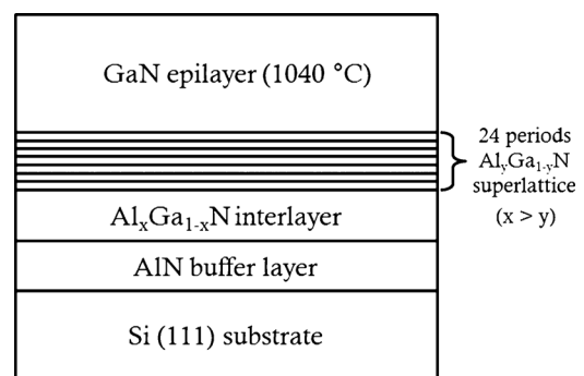
FIG. 1. Schematic representing the sample structure (Al compound: x > y ).
