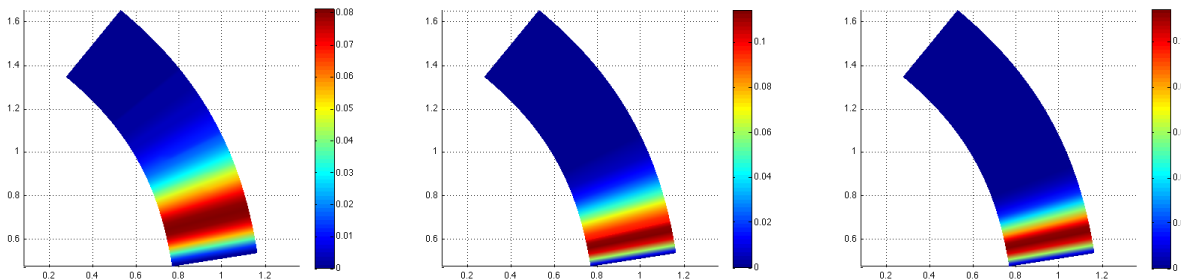
FIGURE 18. Model L: 2D first eigenmode (radial component) for \varepsilon = 10^{-3} and k = 15 , \varepsilon = 3 \cdot 10^{-4} and k = 26 , \varepsilon = 10^{-4} and k = 43 . Represented on \omega^{0.2} .
