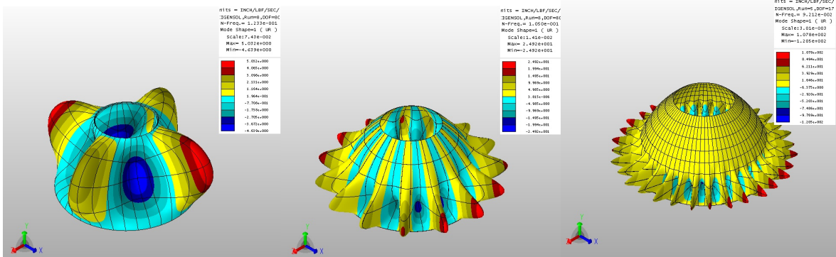
FIGURE 17. Model L: 3D first eigenmode (radial component) for \varepsilon = 10^{-2}, 10^{-3}, 10^{-4} .
