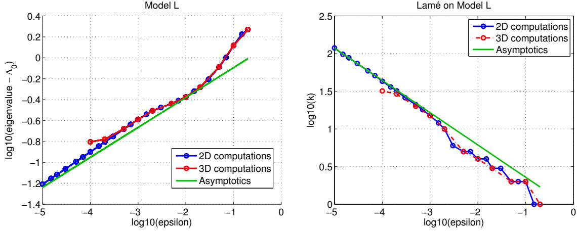
FIGURE 16. Model L: Difference \tilde{\lambda}_1^\varepsilon - \Lambda_0 and associated azimuthal frequency k(\varepsilon) .
