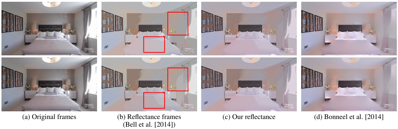
Figure 5: The intrinsic decomposition problem is inherently unstable. Processing the original frames (a) using the single-image technique of Bell et al. [2014] produces reflectance frames with temporal inconsistencies (emphasized in red) (b). In spite of having no knowledge about the intrinsic image problem, our approach produces stabilized reflectance frames (c), that are qualitatively similar to the interactive solution of Bonneel et al. [2014] that explicitly encodes temporal coherence.
