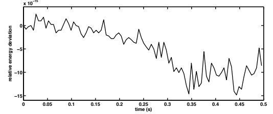
Figure 2: Convergence curve
