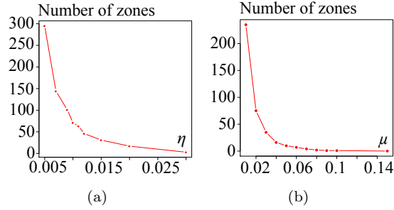
FIGURE 6. Variations of the number of \eta BR or \mu GB minus the number of \lambda FZ versus the parameter \eta or \mu in image "woman face" for \lambda = 0.005 (Chi-squared distance d_{\chi^2} ). (a) \eta BR . (b) \mu GB .
