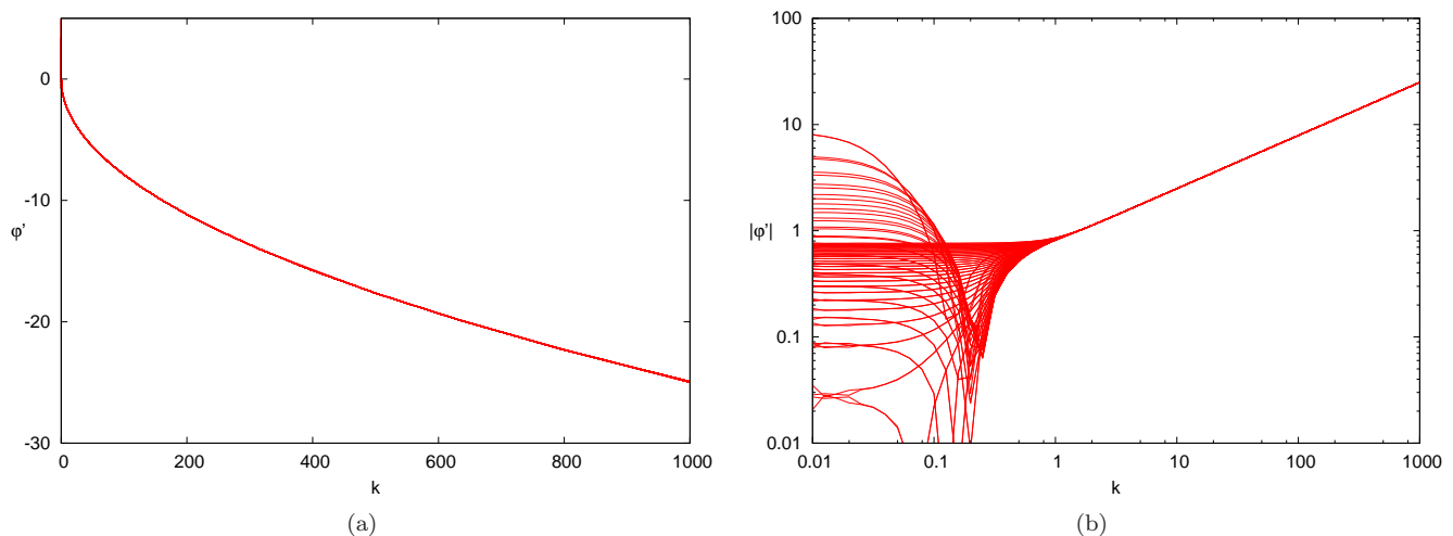
FIG. 3. The behavior of \varphi'(k) = \partial_k \varphi(k) as a function of k is presented for generic superselection sectors (without differentiating between branches corresponding to different values of \epsilon ). (a) presents its behavior in linear scale, whereas (b) shows its absolute value in logarithmic scale.
