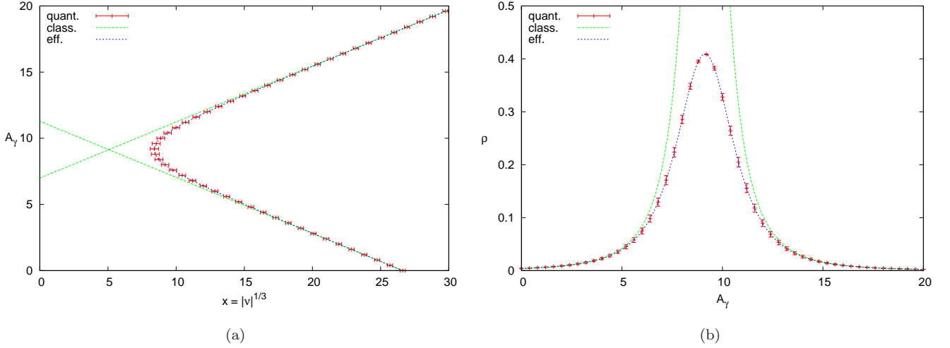
FIG. 2. The expectation values of the observables \widehat{x}|_{A_\gamma} = |\nu|_{A_\gamma}^{1/3} and \widehat{\rho}|_{A_\gamma} evaluated for the wave packet presented in Fig. 1 are compared with the classical trajectories and the evolution predicted by the effective dynamics discussed in Sec. V.
