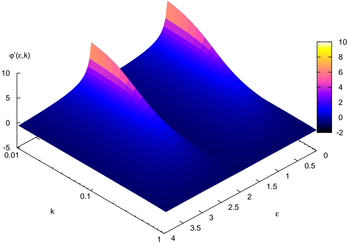
FIG. 4. The behavior of \varphi' = \partial_k \varphi as a function of both k and the superselection sector label \epsilon is shown for small k .
