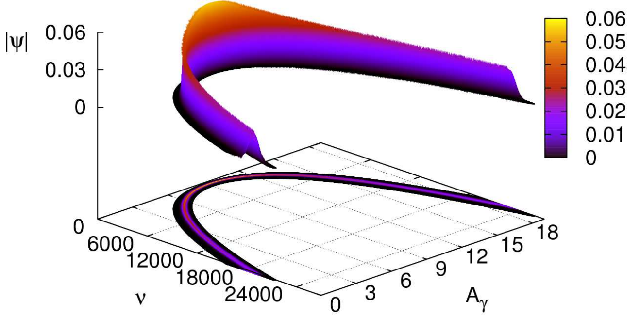
FIG. 1. An example of a physical state: forward evolution of the Gaussian (3.27) packet peaked about \Pi_\gamma \approx 83.3 (G\sqrt{\hbar})^{-1} and (at initial time A_\gamma = 0 ) about \nu \approx 1.8 \times 10^4 .
