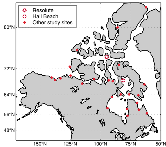
Figure 1. Study sites in the Canadian Arctic. Resolute and Hall Beach are highlighted as they are selected as examples in other figures.
