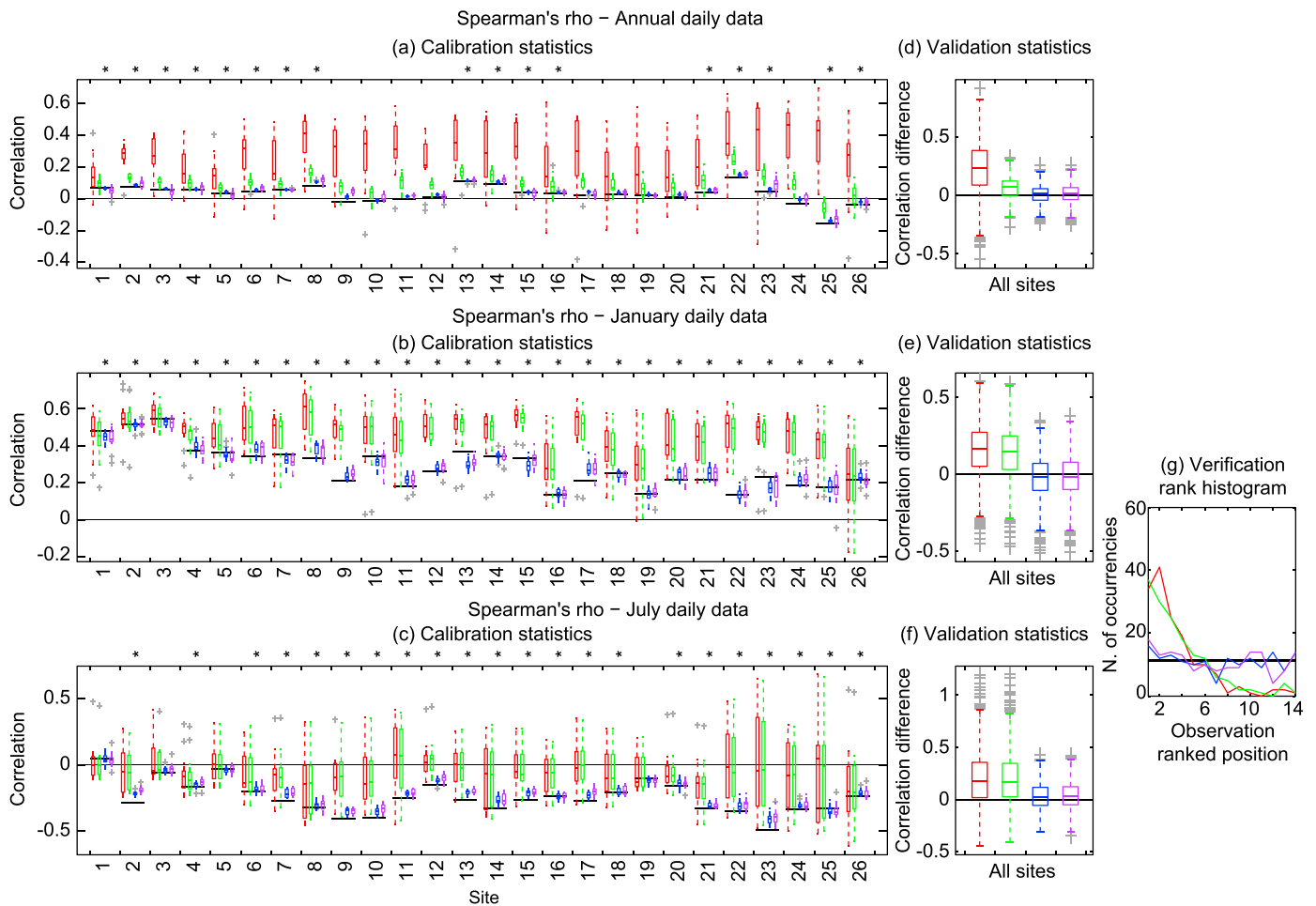
Figure 5. T_{\text{mean}}-Pr correlation results. (a–c) Boxplots show Spearman’s rho values over the full calibration period in observations (black), and DirectSim (red), 1Dqm (green), 2Dqm (blue), and 2Dcopula (violet) scenarios at each site for the ensemble of simulations. Stars on the top of Figures 5a–5c indicate that the correlation in the observations is significant ( p < 0.001 ). (d–f) Boxplots show differences in Spearman’s rho values between observations and scenarios over the three validation periods at all sites for the ensemble of simulations (1014 values per box). (g) The verification rank histogram based on monthly values. Each colored line represents the frequency distribution of 156 cases (three periods \times 26 sites \times two months), whereas the horizontal black line represents the ideal distribution.
