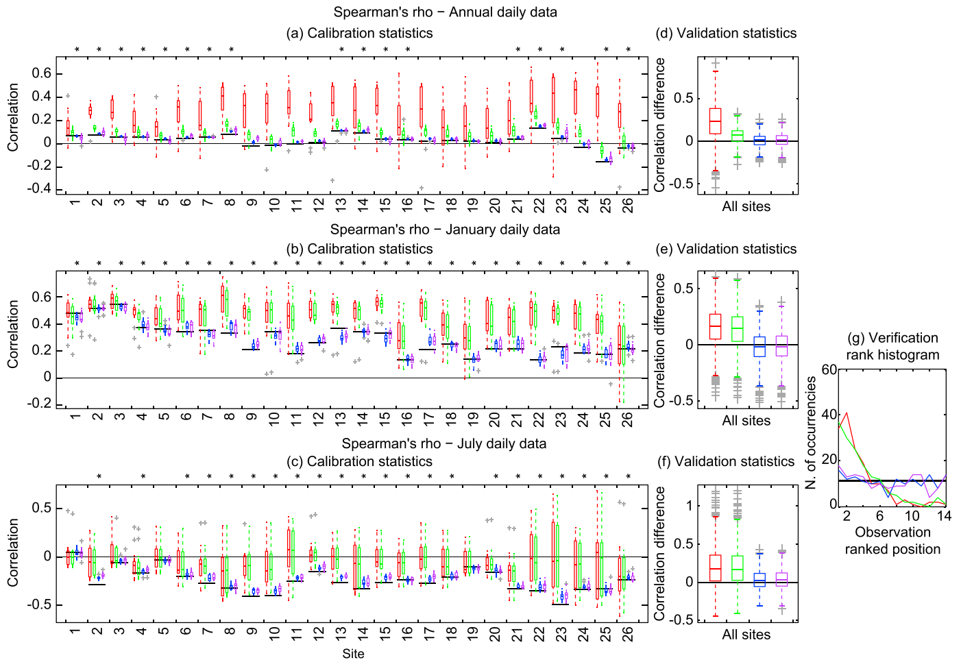
Figure 5. T_{\text{mean}}-Pr correlation results. (a–c) Boxplots show Spearman’s rho values over the full calibration period in observations (black), and DirectSim (red), 1Dqm (green), 2Dqm (blue), and 2Dcopula (violet) scenarios at each site for the ensemble of simulations. Stars on the top of Figures 5a–5c indicate that the correlation in the observations is significant ( p < 0.001 ). (d–f) Boxplots show differences in Spearman’s rho values between observations and scenarios over the three validation periods at all sites for the ensemble of simulations (1014 values per box). (g) The verification rank histogram based on monthly values. Each colored line represents the frequency distribution of 156 cases (three periods \times 26 sites \times two months), whereas the horizontal black line represents the ideal distribution.
