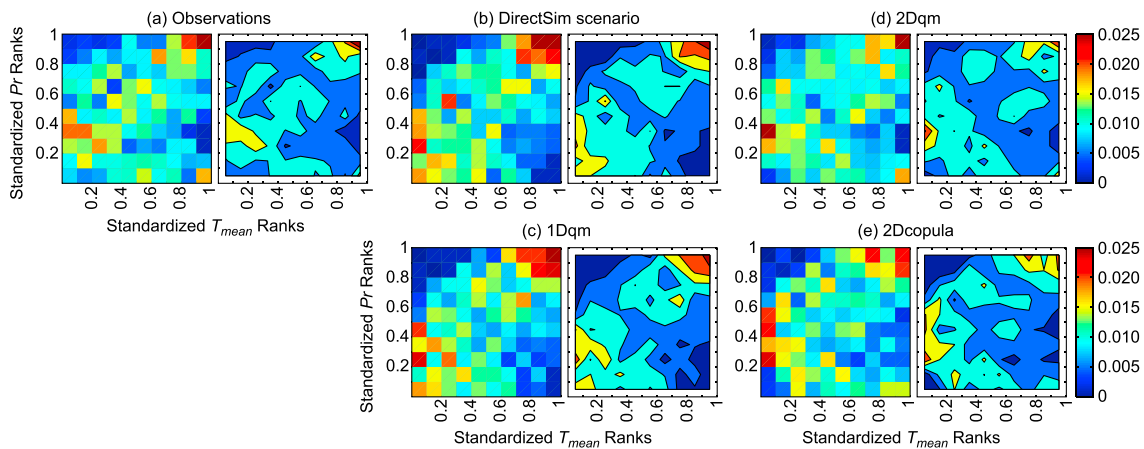
Figure 7. Empirical copula densities of both observed and scenario daily January T_{mean} and P_r data over the full calibration period. Copulas for one model (MIROC-ESM) and one site (Resolute) are shown as an example. (a) Observations, (b) DirectSim scenario, (c) 1Dqm, (d) 2Dqm, and (e) 2Dcopula. Two visualizations are visible for each copula: grid plot and contour plot based on the gridded one. Days without rain in each time series are altered by adding a small noise uniformly distributed ranging from 0 mm to the minimum precipitation value. This last step is iterated 100 times, and the average of 100 empirical copulas is plotted.
