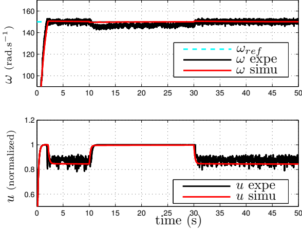
Fig. 2. Comparison of simulation and experimental results for PID controller and \tau = 0 s
