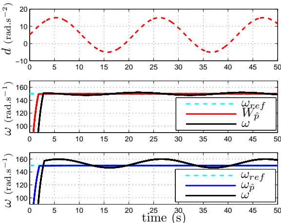
Fig. 6. Simulation results with \tau = 1 s Top: Time-varying Disturbance – Middle: STA with new prediction – Bottom: STA with standard prediction.
