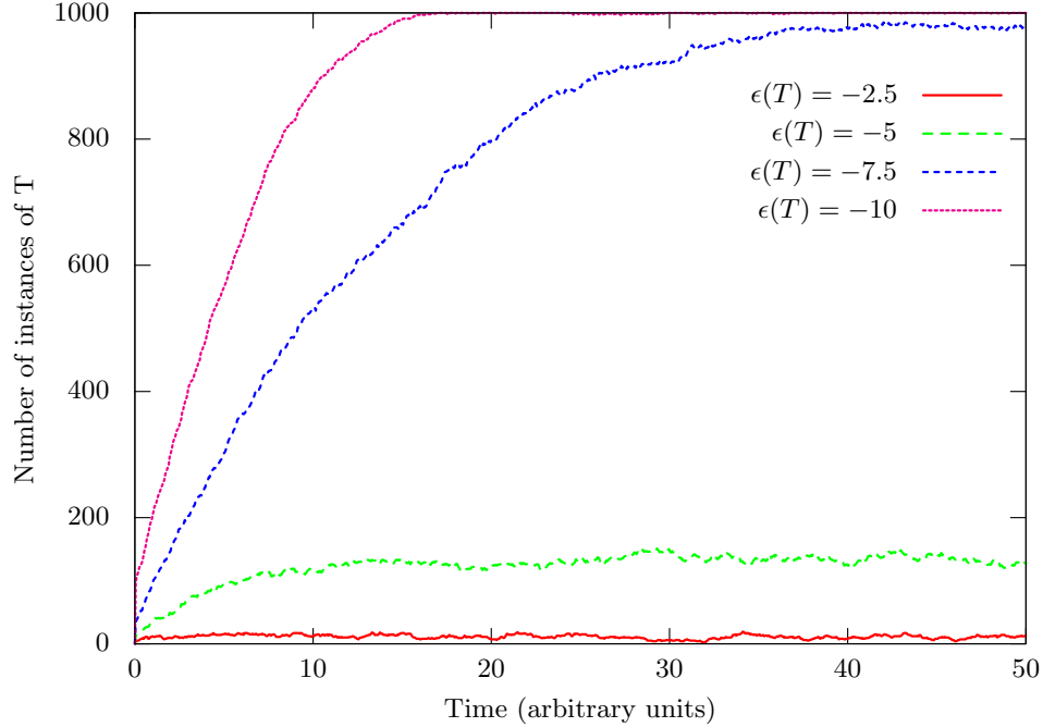
Figure 4: Trajectories for T = \cdot 123 \cdot when \epsilon(T) varies (this value is set by changing the value of parameter ‘t’ in the KaSim file).
