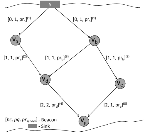
Fig. 2: Beacon messages include: hop count ( hc ), path quality ( pq ) and pressure ( pr ).
