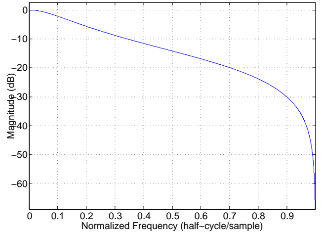
Fig. 2. Profile of low-pass filter (filter response, in dB, as a function of normalized frequency, in half-cycles/sample).
