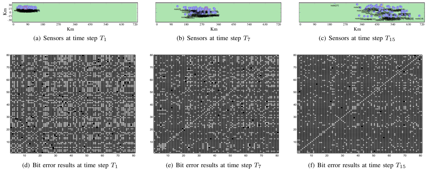
Fig. 6. Sample OMNeT++ mobility simulation. Subfigures (a), (b) and (c) depict the position progression at three different time scale events of eighty sensors randomly dispersed on the axis of a meandering current. Subfigures (d), (e) and (f) plot a bidimensional communication map, in which every square represents the associated bit error ratio during the data transmission of any two sensors at a given time step. White squares represent data transfers with a bit error ratio below 33%. Gray squares represent bit error ratios between 33% and 77%. Black squares represent bit error ratios higher than 77%.
