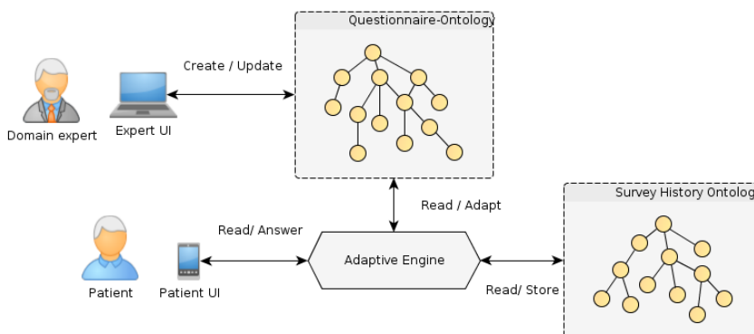
Fig. 1. Information Gathering System architecture
