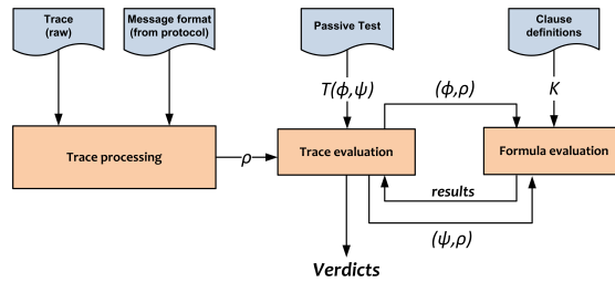
Fig. 1. Testing framework of Datamon
