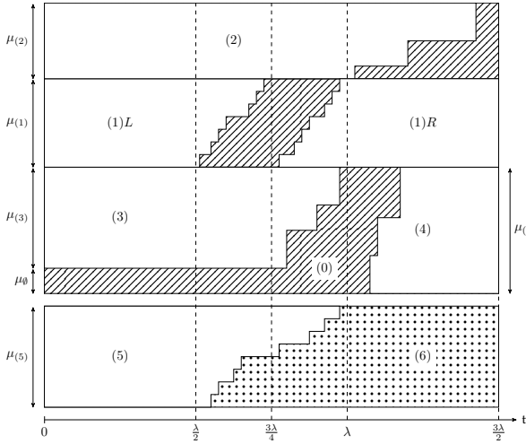
Fig. 1: Structure of the schedule. The number of processors used by set (i) is denoted by \mu_{(i)} . The number of CPUs below set (3) is denoted by \mu_0 .
