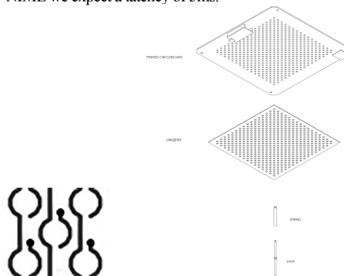
Figure 3 Left: Sample of the PCB grid showing the two semi-circles. Left supplies and right measures voltage. Right: Technical setup for Tingle
