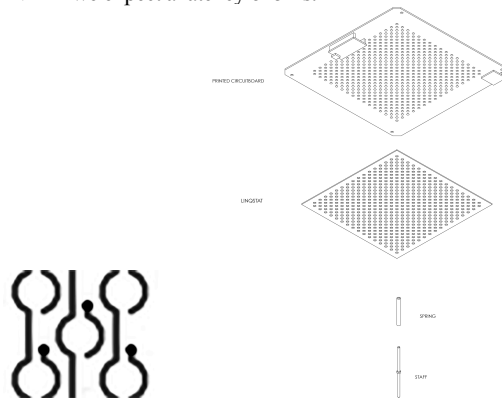
Figure 3 Left: Sample of the PCB grid showing the two semi-circles. Left supplies and right measures voltage. Right: Technical setup for Tingle
