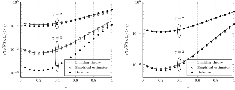
Figure 3: False alarm rate P(\sqrt{N}T_N(\rho) > \gamma) , N = 20 (left), N = 100 (right), p = N^{-\frac{1}{2}}[1, \dots, 1]^T , [C_N]_{ij} = 0.7^{|i-j|} , c_N = 1/2 .
