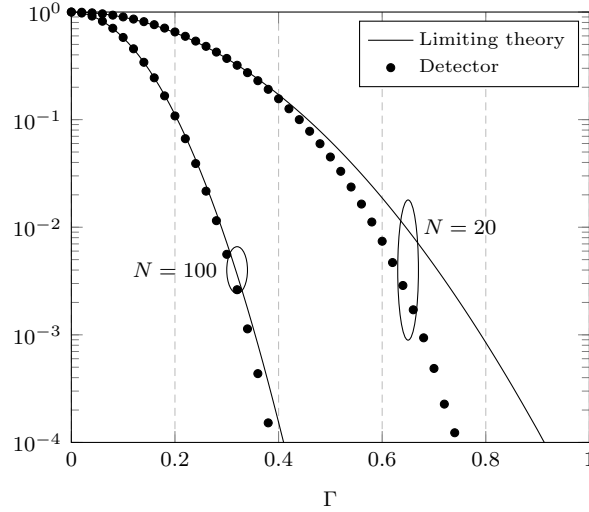
Figure 4: False alarm rate P(T_N(\rho) > \Gamma) for N = 20 and N = 100 , p = N^{-\frac{1}{2}}[1, \dots, 1]^T , [C_N]_{ij} = 0.7^{|i-j|} , c_N = 1/2 .
