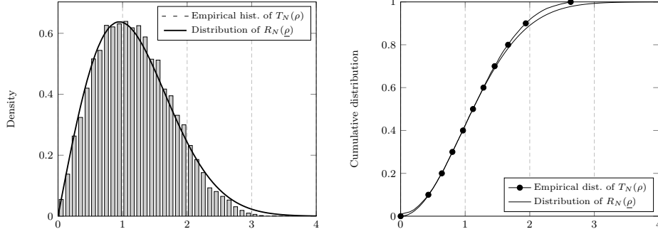
Figure 1: Histogram distribution function of the \sqrt{N}T_N(\rho) versus R_N(\rho) , N = 20 , p = N^{-\frac{1}{2}}[1, \dots, 1]^T , [C_N]_{ij} = 0.7^{|i-j|} , c_N = 1/2 , \rho = 0.2 .
