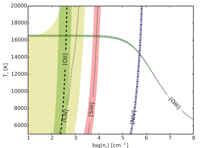
Figure 7. Range of electron density and temperature allowed by our emission line ratio diagnostics. Most diagnostics agree on a temperature of \sim 16\,500 \text{ K} and an electron density of \sim 300 \text{ cm}^{-3} . The discrepancy of the N IV] \lambda \lambda 1483, 86 diagnostic can be due to its higher ionization energy, which would limit it to probe higher density regions (closer to the ionizing source).
