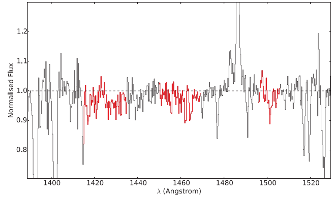
Figure 9. Equivalent widths of faint absorption features were estimated in three spectral windows (in red) of the normalized spectrum (in black). These were used as direct stellar metallicity estimators, following the work from Sommariva et al. (2012). Applying their calibrations, we derive a low stellar metallicity for the first two windows (F1425 and F1460 indices) of 0.0424 and 0.0678 Z_{\odot} , respectively.
