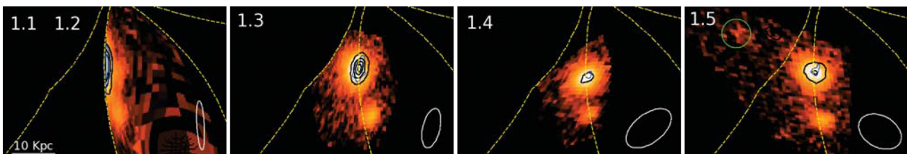
Figure 3. Source plane reconstruction of the \text{Ly}\alpha line image. Dashed yellow: caustic lines. Blue contours: \text{C III]} line image reconstruction. Black contours: continuum near \text{Ly}\alpha image reconstruction. The ellipses on the lower right corners correspond to the source plane PSF, obtained by reconstructing the 2D Moffat profile of the measured seeing (at the wavelength of \text{Ly}\alpha ) into the source plane. The small differences between the source plane images are well explained by the different PSF shapes. Note that images 1.1 and 1.2 are radial images and only cover the western half of the source.
