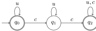
Fig. 4: Property that can be enforced by blocking all controllable events c , thus outputting only the uncontrollable ones u .
