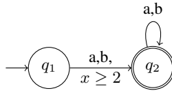
Fig. 6: A timed property enforceable only if \Sigma_u = \emptyset .
