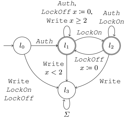
Fig. 8: Property modelling writes on a shared storage device
