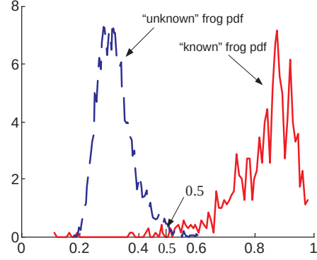
Figure 7: PDF of the scores of known frogs with unknown frogs and PDF of the scores of known frogs with themselves.
