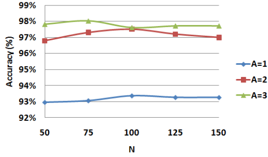
Figure 6: PCA accuracy as A, N vary.
