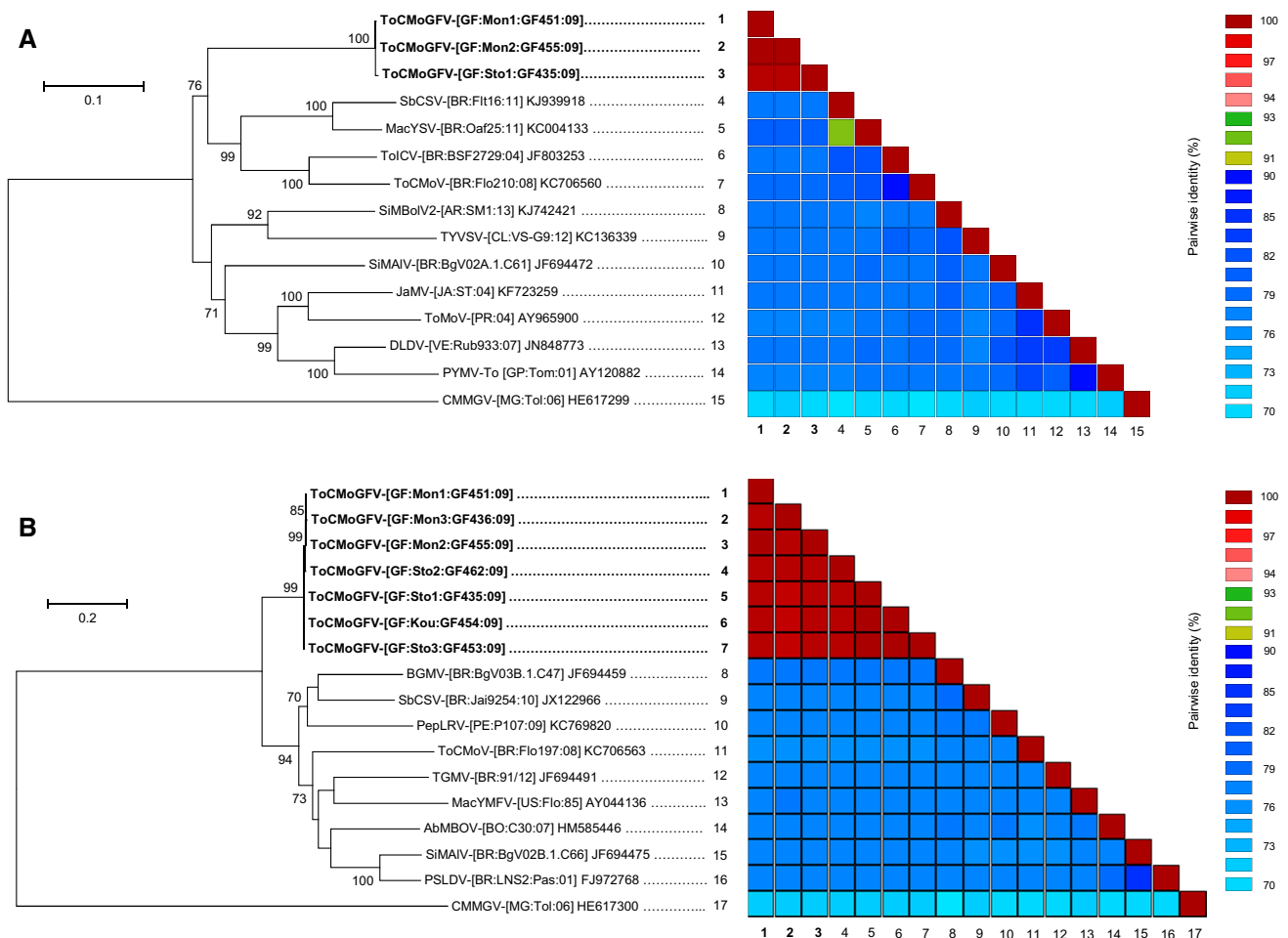
Fig. 1 Maximum-likelihood phylogenetic trees and colour-coded matrix of pairwise nucleotide sequence identity inferred from alignments of complete DNA-A (A) and DNA-B (B) sequences of ToCMoGFV and representative New World bipartite begomoviruses. Only bootstrap values at nodes higher than 70 % are displayed (1000 replicates). The scale bar represents the genetic distance. The trees
