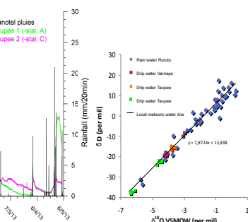
Figure 6. \delta^{18}\text{O} and \delta\text{D} (‰ vs. VSMOW) of rainwater and dripwaters in Taupee and Vairepo caves.
