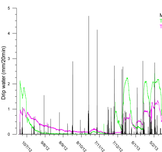
Figure 5. Rainfall (black) and drip rate under two stalactites (green and pink) in Taupee cave, recorded every 20 min.
