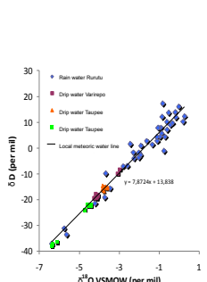
Figure 6. \delta^{18}\text{O} and \delta\text{D} (‰ vs. VSMOW) of rainwater and dripwaters in Taupee and Vairepo caves.
