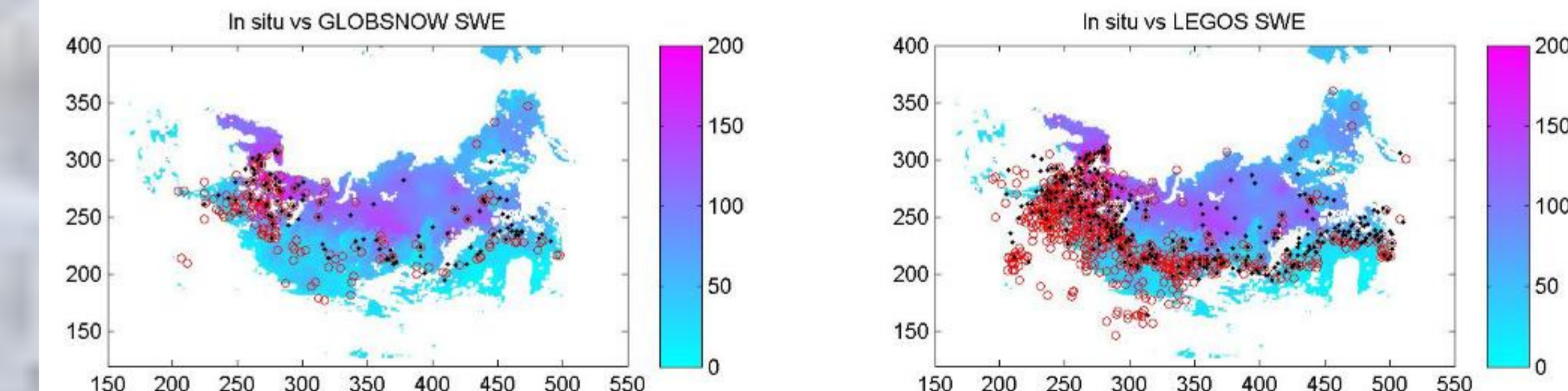
Example of SWE products for Feb. 1996 ; The comparison has been performed over more than 1000 in situ stations.
