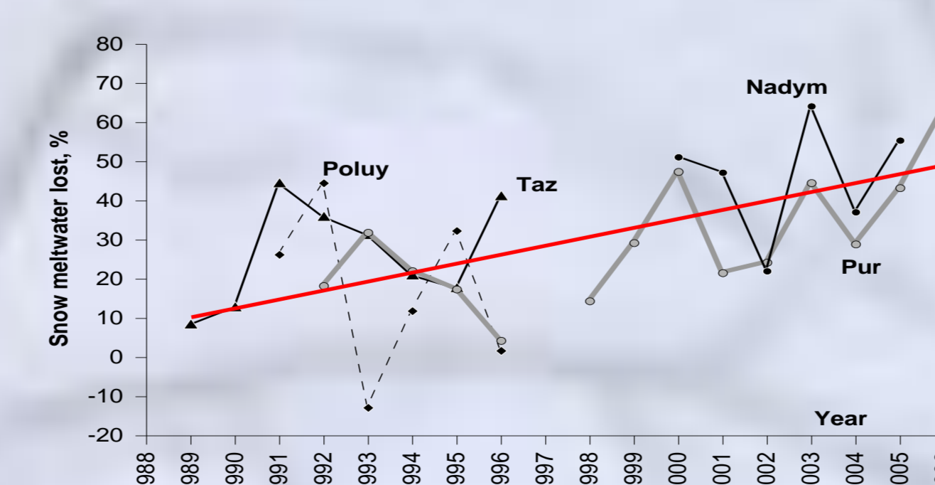
Temporal evolution of difference between snow volume (from SSM/I) and spring flood (from in situ), i.e. % of snow lost, for 4 NW Siberian catchments
