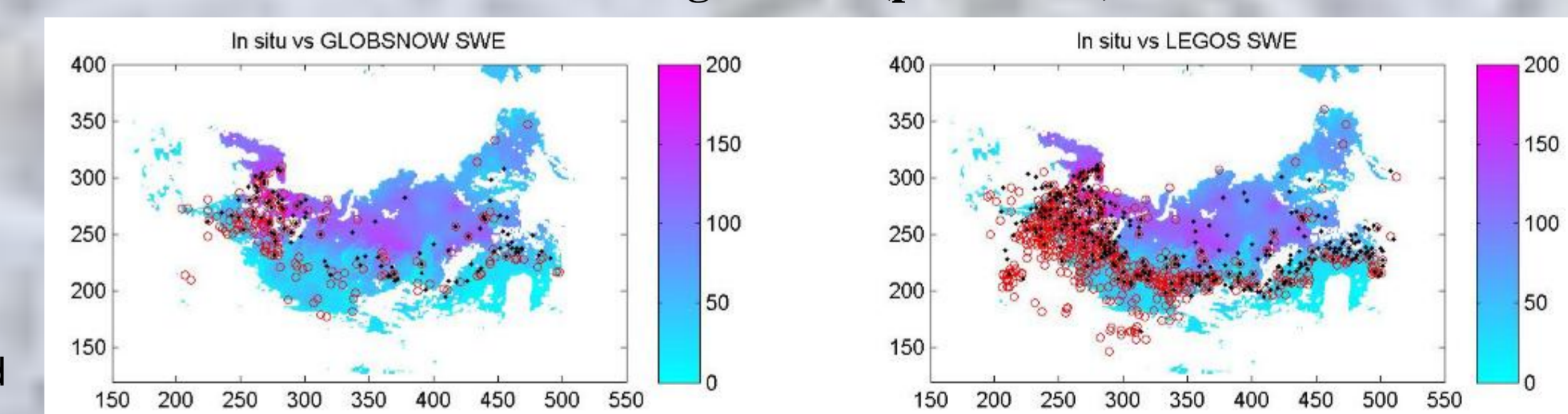
Example of SWE products for Feb. 1996 ; The comparison has been performed over more than 1000 in situ stations.
