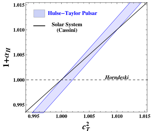
FIG. 2: Combined constraints in the (c_T^2, \alpha_H) parameter space for the linear branch of solutions (14). The (tight) bound the Cassini measurement [20] (black curve) and the light-blue stripe corresponding to the Hulse-Taylor pulsar bound obtained from the top panel. Within Horndeski theories, because G_N = c_T^2 G_{\text{gw}} , the bound (6) turns into a slight preference for superluminal propagation.
