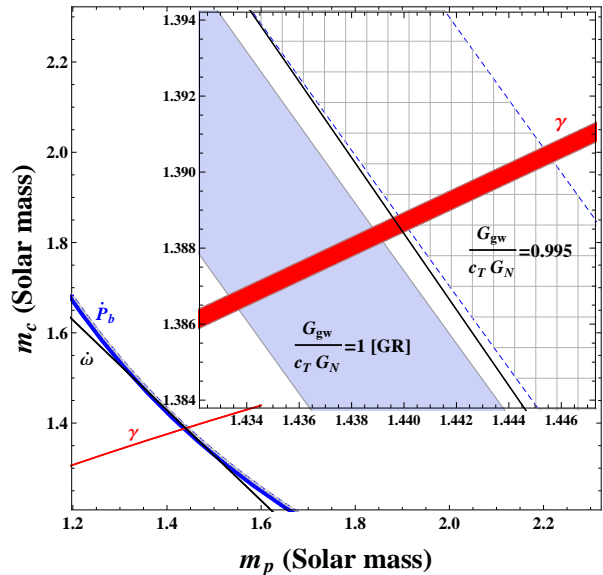
FIG. 1: Mass-mass diagram for PSR B1913+16 (the Hulse-Taylor pulsar) based on the post-Keplerian parameters \dot{\omega} (black), \gamma (red) and \dot{P}_b (blue). Varying the combination c_T G_{\text{gw}}/G_N amounts to shifting the 1- \sigma stripe of \dot{P}_b .
