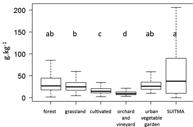
Fig. 2. Distribution of total organic carbon in French topsoils according to land use: forest ( n = 582 ), grassland ( n = 623 ), cultivated ( n = 820 ), orchard and vineyard ( n = 48 ), urban vegetable garden ( n = 104 ) and SUITMA ( n = 229 ). Band inside the box represent the median. Bottom and top of the box are the first and third quartiles. The whiskers indicate the lowest datum within 1.5 interquartile range of the lower quartile, and the highest datum within 1.5 interquartile range of the upper quartile. Lower case letters indicate significant differences between land use.
