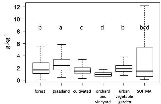
Fig. 3. Distribution of total nitrogen in French topsoils according to land use: forest ( n = 582 ), grassland ( n = 623 ), cultivated ( n = 820 ), orchard and vineyard ( n = 48 ), urban vegetable garden ( n = 104 ) and SUITMA ( n = 219 ). Band inside the box represent the median. Bottom and top of the box are the first and third quartiles. The whiskers indicate the lowest datum within 1.5 interquartile range of the lower quartile, and the highest datum within 1.5 interquartile range of the upper quartile. Lower case letters indicate significant differences between land use.
