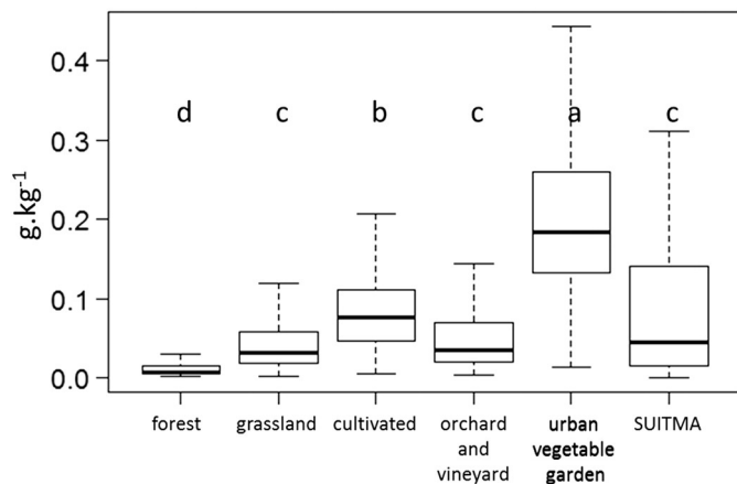
Fig. 5. Distribution of available phosphorus (Olsen method) in French topsoils according to land use: forest ( n = 582 ), grassland ( n = 623 ), cultivated ( n = 820 ), orchard and vineyard ( n = 48 ), urban vegetable garden ( n = 104 ) and SUITMA ( n = 173 ). Band inside the box represent the median. Bottom and top of the box are the first and third quartiles. The whiskers indicate the lowest datum within 1.5 interquartile range of the lower quartile, and the highest datum within 1.5 interquartile range of the upper quartile. Lower case letters indicate significant differences between land use.
