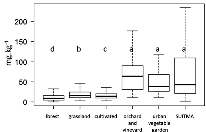
Fig. 7. Distribution of total copper in French topsoils according to land use: forest ( n = 582 ), grassland ( n = 623 ), cultivated ( n = 820 ), orchard and vineyard ( n = 48 ), urban vegetable garden ( n = 104 ) and SUITMA ( n = 238 ). Band inside the box represent the median. Bottom and top of the box are the first and third quartiles. The whiskers indicate the lowest datum within 1.5 interquartile range of the lower quartile, and the highest datum within 1.5 interquartile range of the upper quartile. Lower case letters indicate significant differences between land use.
