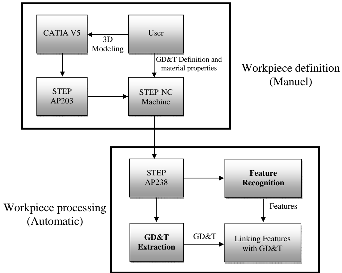
Fig. 2. Architecture of the proposed system for technical data extraction and feature recognition
