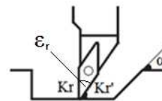
Fig. 6. Geometry of a recess feature
