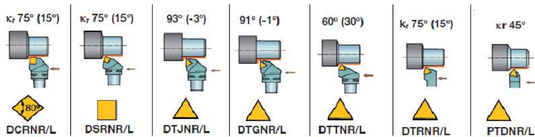
Fig. 4. Example of holders and inserts of B class of operations
