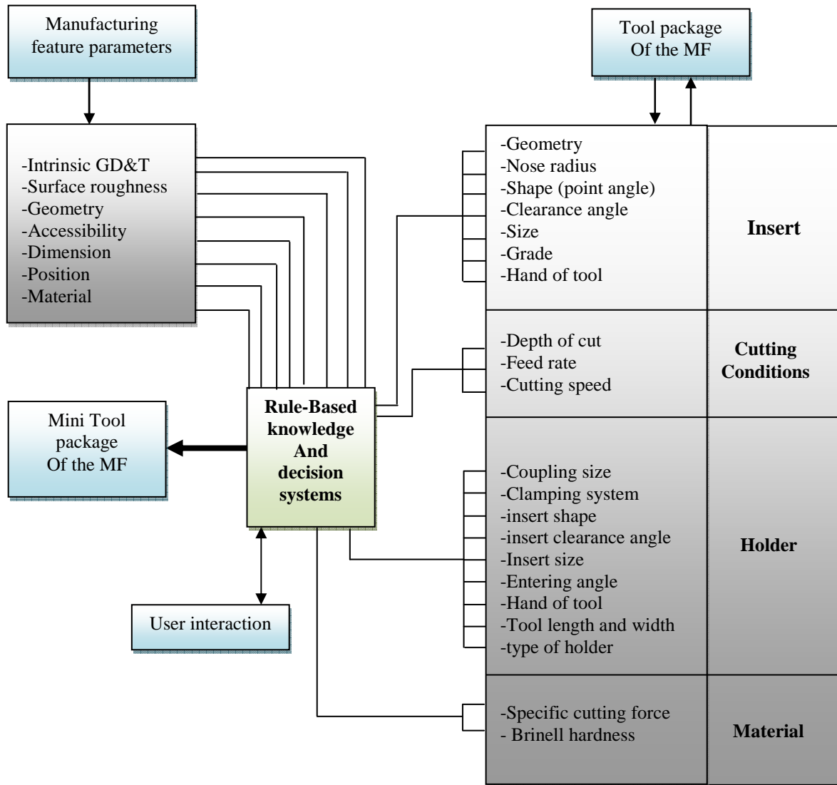
Fig. 5. Flowchart of the microscopic tool parameters choice
