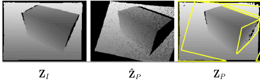
Fig. 3. An intuitive example of forward estimation. The depth frame \hat{\mathbf{Z}}_P is predicted from \mathbf{Z}_I as the frame captured at P-frame's viewpoint virtually. After comparing \hat{\mathbf{Z}}_P and \mathbf{Z}_P , the newly observed information in \mathbf{Z}_P is outlined in yellow.
