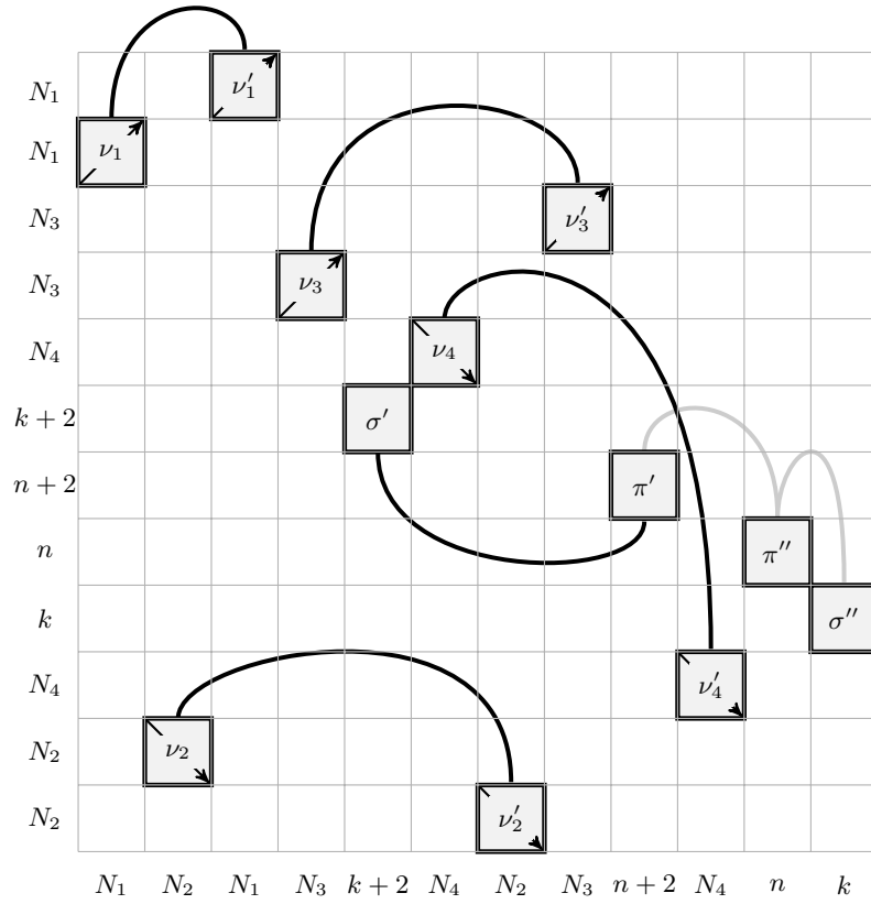
Fig. 3. Schematic representation of the permutation \mu used in Proposition 4. Black edges denote the presence of at least one edge between two bunches of vertices in K_\mu . Grey edges denote edges that are only considered in the forward direction of the proof.
