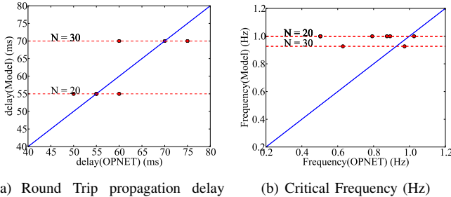
(a) Round Trip propagation delay (ms) at critical frequency.
