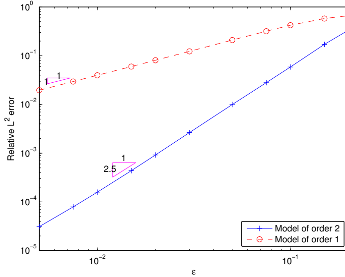
FIG. 4.3. Relative \mathbf{L}^2 errors of the solutions \mathbf{E}_0, \mathbf{E}_\varepsilon^1 of the equivalent models of order 1 and 2 versus the thickness \varepsilon (higher frequency \omega = \pi ).
