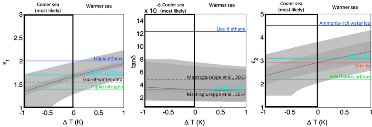
Figure 9. Model fitting results as a function of the temperature difference \Delta T (in K) between Ligeia Mare and the surrounding lands for (left) the dielectric constant of the liquid \epsilon_1 , (middle) the loss tangent of the liquid \tan \delta , and (right) the dielectric constant of the seafloor \epsilon_2 . These results were obtained assuming a smooth sea surface and an isothermal sea. The associate reduced chi-square values are all \sim 1.7 . The dark gray shaded areas show the upper and lower confidence limits of the 90% confidence interval accounting for the relative error on radiometry measurements. The light gray shaded areas show the upper and lower confidence limits of the 90% confidence interval accounting for both the relative and absolute errors on radiometry measurements. The black rectangles highlight the most likely results (obtained for \Delta T \leq 0 K), the hypothesis of the sea warmer than its surrounding being highly implausible as explained in section 4.1. The values of the dielectric constant and loss tangent of materials relevant to Titan’s surface as well as results from other observations are indicated for comparison.
