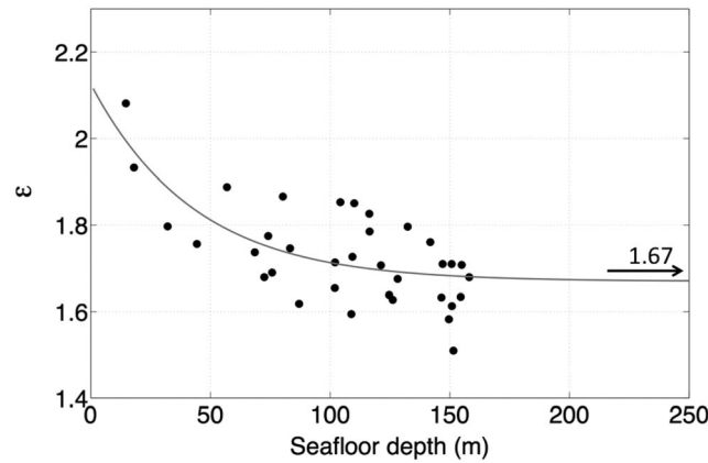
Figure 10. Bulk dielectric constant of the column of material sensed by the Cassini radiometer during the T91 altimetry pass as a function of the seafloor depth inferred from radar active data. The gray line displays the best fit model (in the smooth case assuming \Delta T = 0 K) as derived in section 4.2.
