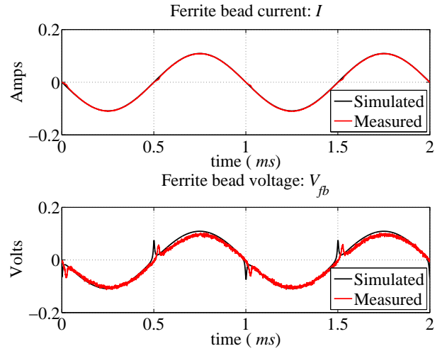
Fig. 11. Ferrite bead current and voltage.
