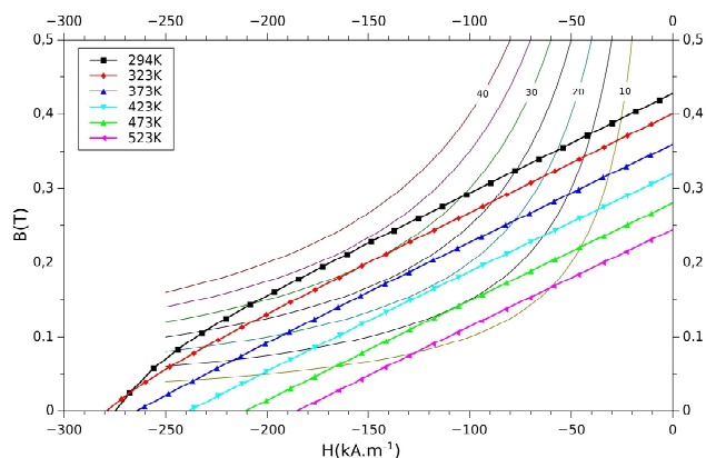
Fig. 14. Demagnetization curves, the lines are the (BH)=\text{constant} curves ( \text{kJ.m}^{-3} ). Over 323 K (50°C), the coercivity field in the B(H) plan is \mu_0 H_{cB} = J_R .
