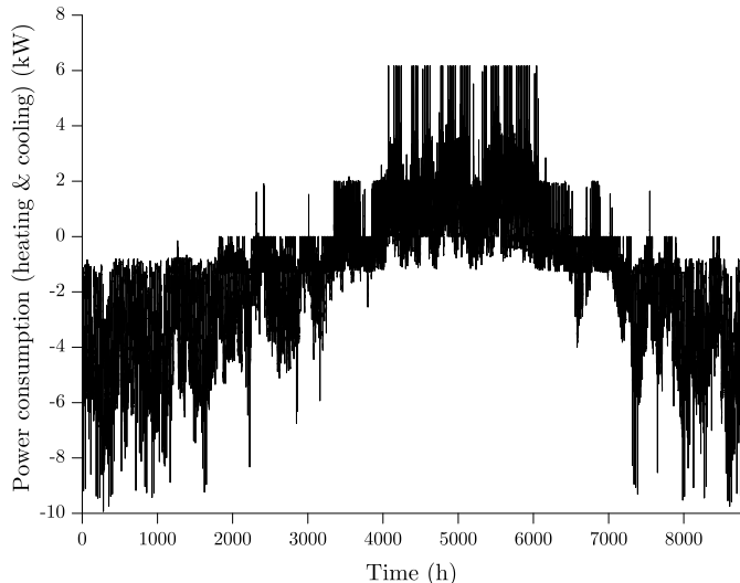
Figure 5: Hourly power consumption for heating and cooling in the single-storey house located in Perpignan (Perpignan-Méditerranée agglomération community, Languedoc-Roussillon, France) (kW). When power consumption is negative (respectively positive), heating (respectively cooling) mode is on.
